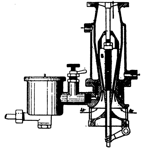
DECAUVILLE CARBURETER, SHOWING AUTOMATIC MIXTURE REGULATING FLOAT.
